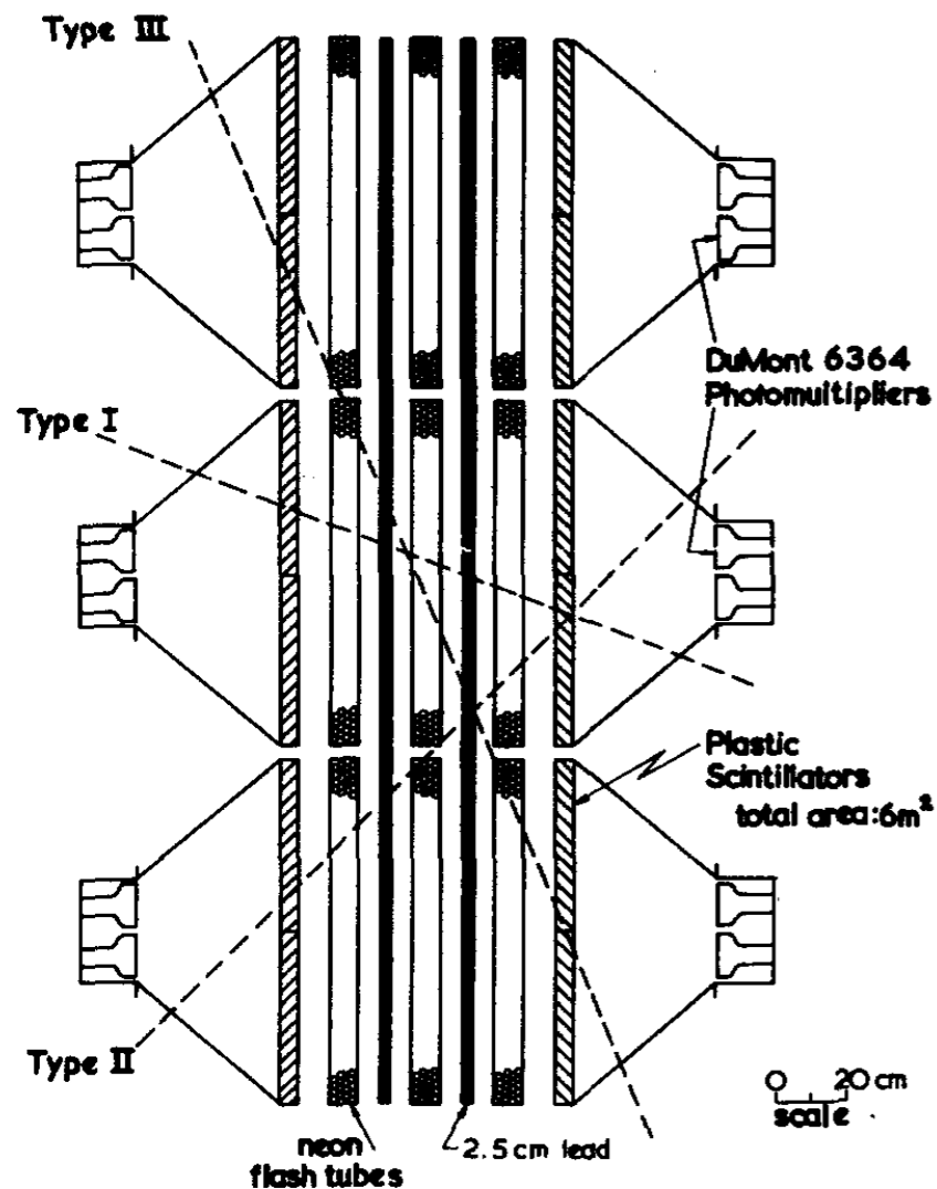
Fig. 1. Neutrino telescope.
