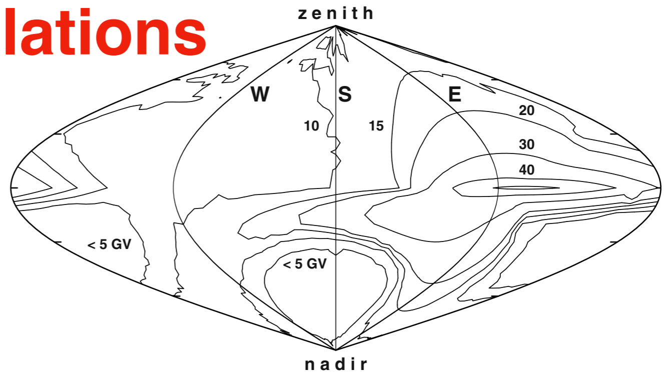
Fig. 7.11. Contour map of the geomagnetic cutoff at Kamioka. Contours connect the directions with equal rigidity cutoffs. East, south and west are indicated and north is split at the edge of the graph.
