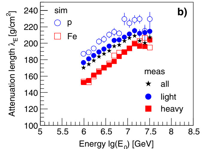
FIG. 4 (color online). Attenuation length \lambda_E as a function of the estimated primary energy. The light and heavy groups in the measurements are compared to simulations of showers induced by primary protons and iron nuclei using CORSIKA with the hadronic interaction model QGSJET 01 (a) and a modified version with lower cross sections and higher elasticity [(b), model 3a in Ref. [25]].
