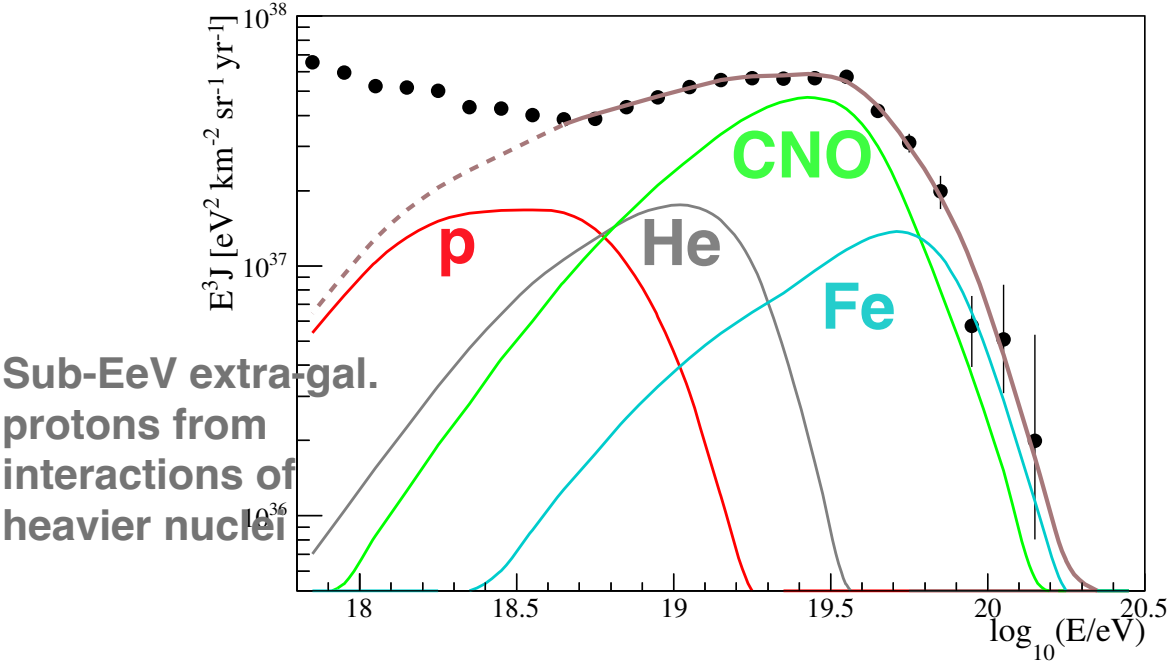
Combined fit of spectrum and composition data as measured by the Pierre Auger Observatory
