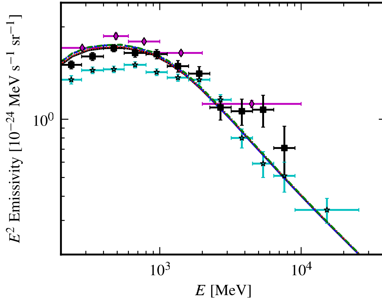
Figure 34. Average emissivity of the local annulus for model S^S Z^4 R^{20} T^{150} C^5 (solid black), S^L Z^6 R^{20} T^{\infty} C^5 (blue dashed), S^Y Z^{10} R^{30} T^{150} C^2 (red dotted), and S^O Z^8 R^{30} T^{\infty} C^2 (green dash-dotted). Shown for comparison are emissivities derived from Fermi -LAT data using a template fitting approach. Cyan stars are from Ackermann et al. (2011b), magenta diamonds are from Abdo et al. (2010d), and black squares are from Abdo et al. (2009b).
