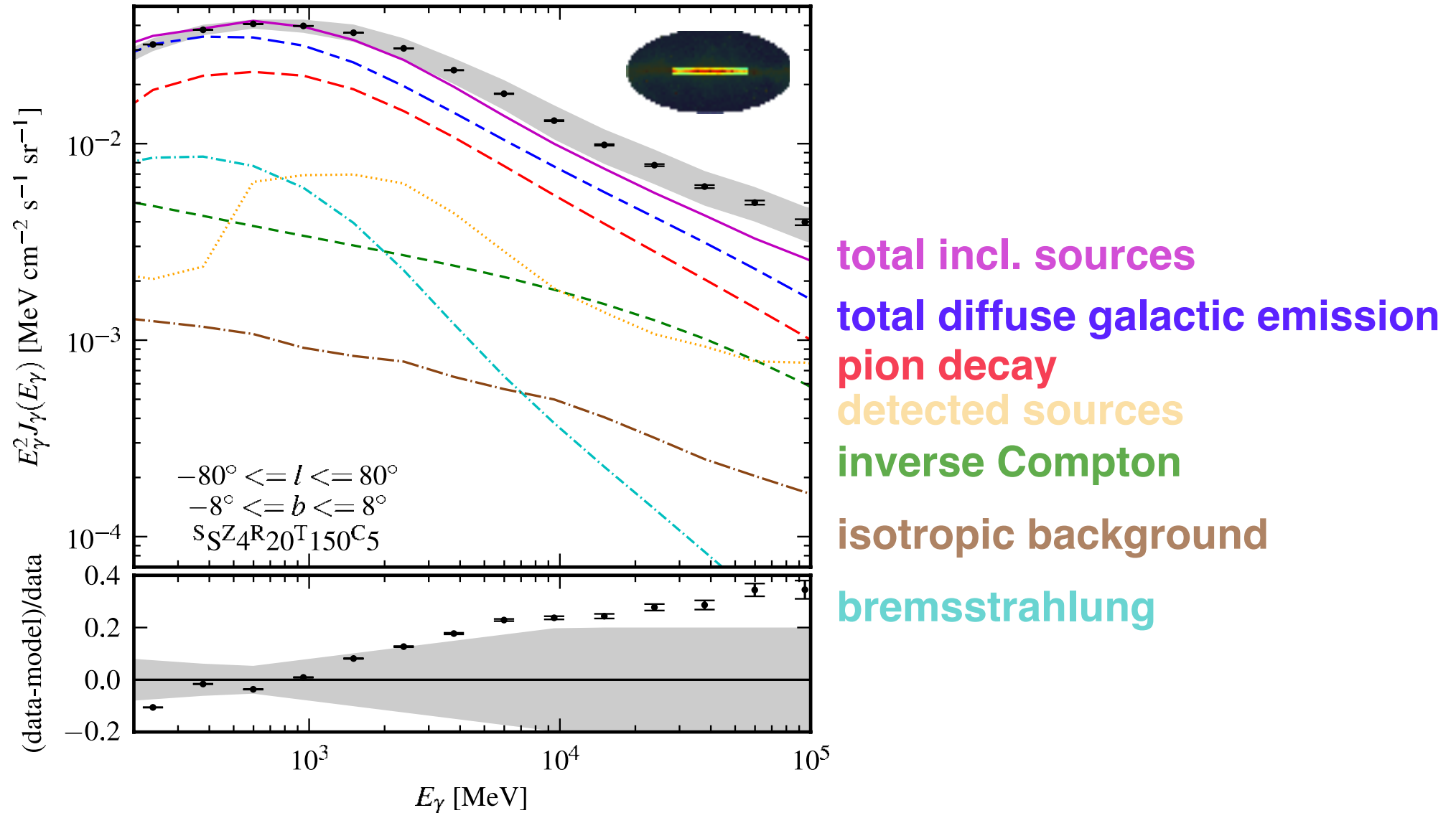
Figure 17. Spectra extracted from the inner Galaxy region for model S_{S^Z}Z_4R_{20}T_{150}C_5 using Pass 7 clean photons. The dip between 10 and 20 GeV is greatly reduced compared to Figure 15. See Figure 12 for legend.
