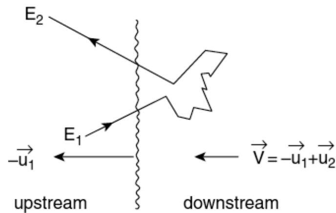
Figure 12.2 Acceleration at a plane shock front.
