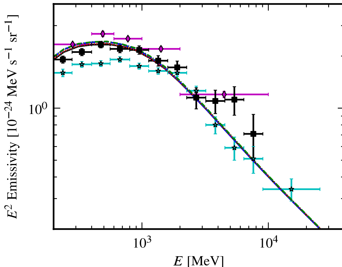
Figure 34. Average emissivity of the local annulus for model S^SZ4R20T150C5 (solid black), S^LZ6R20T\infty C5 (blue dashed), S^YZ10R30T150C2 (red dotted), and S^OZ8R30T\infty C2 (green dash-dotted). Shown for comparison are emissivities derived from Fermi -LAT data using a template fitting approach. Cyan stars are from Ackermann et al. (2011b), magenta diamonds are from Abdo et al. (2010d), and black squares are from Abdo et al. (2009b).
