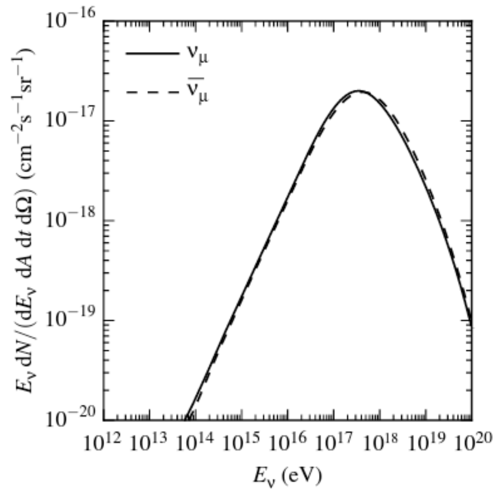
Figure 10.5 Flux of cosmogenic neutrinos from proton interaction with the microwave background [321].
