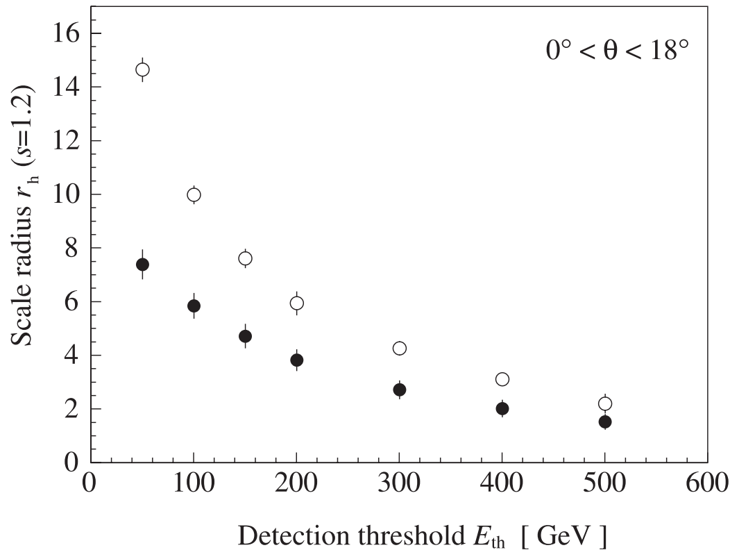
Fig. 15. Hadronic scale radius r_h as a function of detection threshold E_{th} for a fixed shower age of s = 1.2 and 3.4 < \lg N_\mu^{tr} < 3.7 . Filled symbols are for hadronic energy density and open symbols for hadronic particle density.
