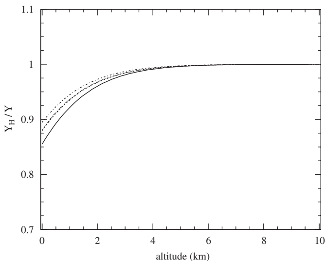
Fig. 5. Ratio of fluorescence yield with measured p'_{H_2O} to the one with p_h = 0 : dashed line 313.6 nm; full line 337.1 nm; dotted line 353.7 nm; dashed-dotted 391.4 nm.
